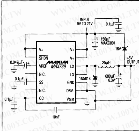
Figure 6. MAX739 +5V Step-Down Application
