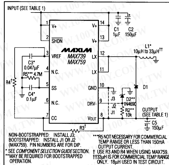
Figure 1b. MAX739/MAX759 Standard Application Circuit (Through-Hole Components)
