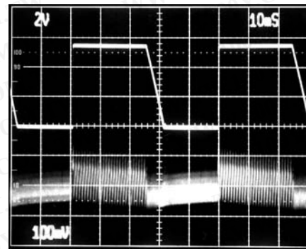
MAX639 LINE-TRANSIENT RESPONSE
