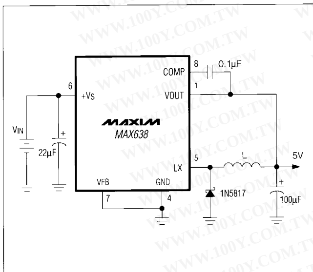
Figure 3. Typical Operating Circuit (Table 1)
