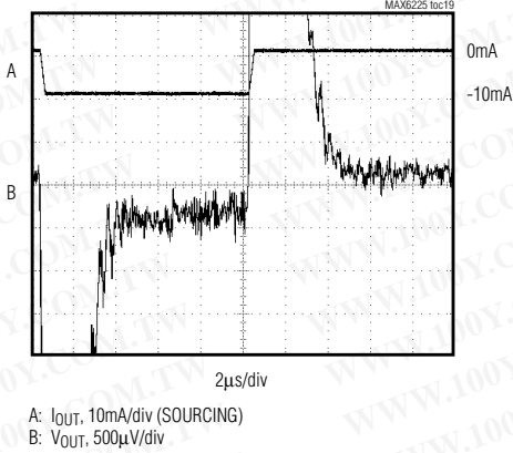
LOAD-TRANSIENT RESPONSE (SOURCING)
