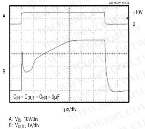
TURN-ON AND TURN-OFF TRANSIENT RESPONSE
