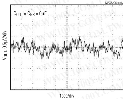
MAX6225 0.1Hz to 10Hz NOISE
