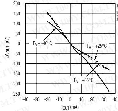
MAX6225 CHANGE IN OUTPUT VOLTAGE vs. OUTPUT CURRENT
