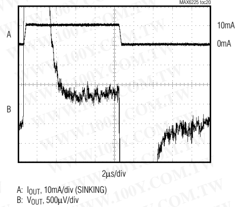
LOAD-TRANSIENT RESPONSE (SINKING)
