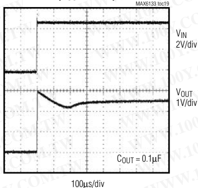
TURN-ON TRANSIENT ( V_{OUT} = 2.5V )
