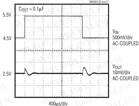
LINE TRANSIENT ( V_{OUT} = 2.5V )
