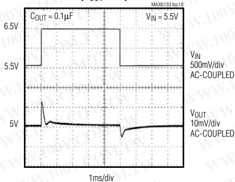
LINE TRANSIENT ( V_{OUT} = 5V )
