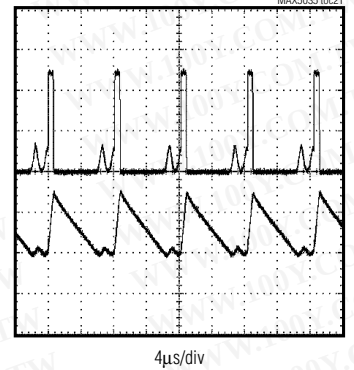
MAX5035DASA LX WAVEFORMS
