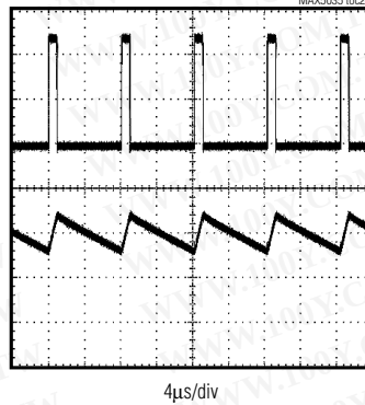
MAX5035DASA LX WAVEFORMS
