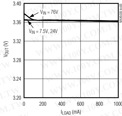
LOAD REGULATION (MAX5035AASA, V OUT = 3.3V)
