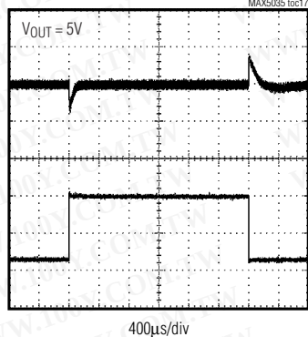
MAX5035DASA LOAD-TRANSIENT RESPONSE
