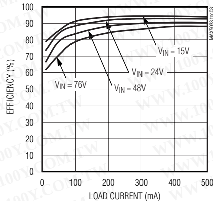
EFFICIENCY vs. LOAD CURRENT (MAX5033CASA, V_{OUT} = 12V )
