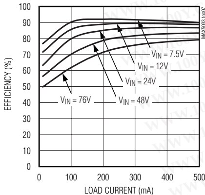
EFFICIENCY vs. LOAD CURRENT (MAX5033BASA, V_{OUT} = 5V )
