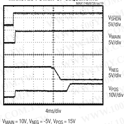
MAX8726 POWER-UP SEQUENCING
