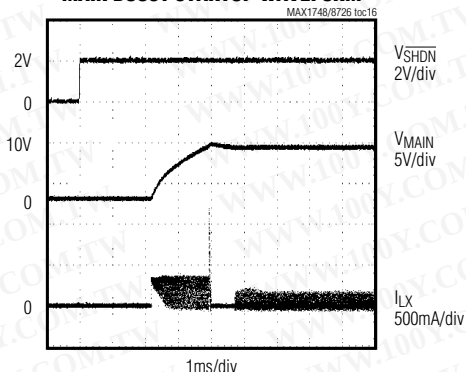
MAIN BOOST STARTUP WAVEFORM
