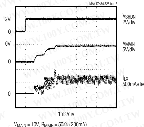
MAIN BOOST STARTUP WAVEFORM WITH LOAD
