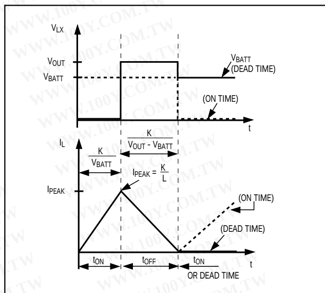
Figure 2. Switching Waveforms
