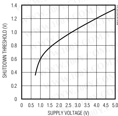
SHUTDOWN THRESHOLD vs. SUPPLY VOLTAGE
