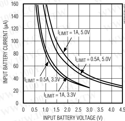
NO-LOAD BATTERY CURRENT vs. INPUT BATTERY VOLTAGE
