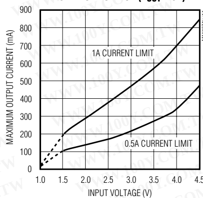
MAXIMUM OUTPUT CURRENT vs. INPUT VOLTAGE ( V_{\text{OUT}} = 5\text{V} )
