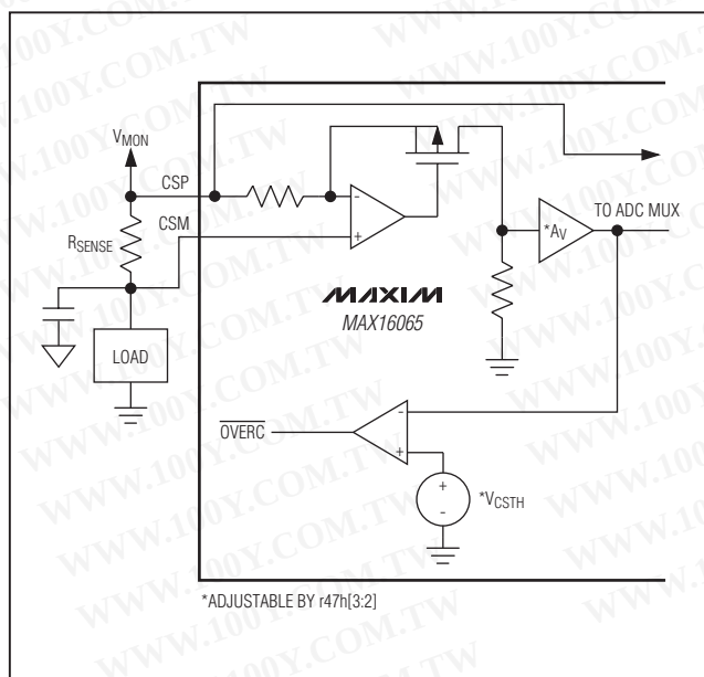
Figure 5. Current-Sense Amplifier
