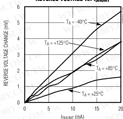
LM4050-5.0V REVERSE VOLTAGE vs. I_{SHUNT}
