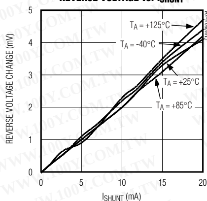
LM4050-2.5V REVERSE VOLTAGE vs. I_{SHUNT}
