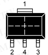
TOP VIEW SOT-223 PACKAGE See Mech. Drawings Section On Website
