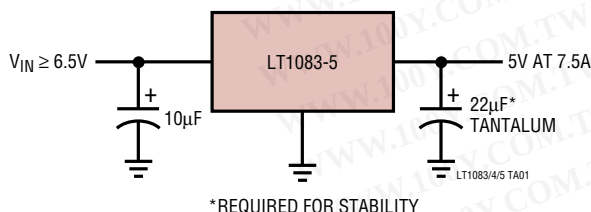
5V, 7.5A Regulator
