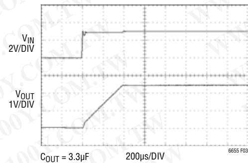
Figure 3. Start-Up Response
