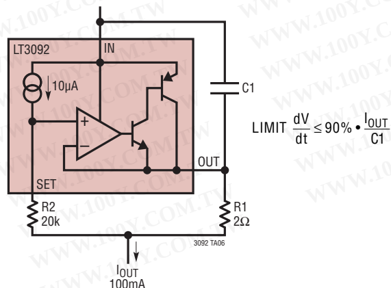
Capacitor Adds Stability, But Limits Slew Rate
