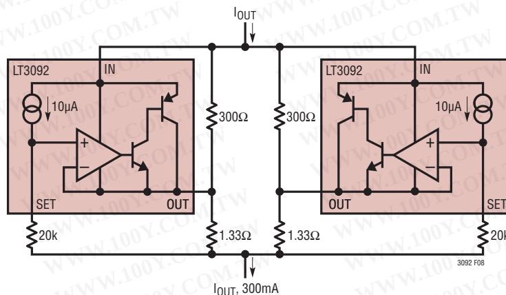
Figure 8. Connect Two LT3092s for Higher Current
