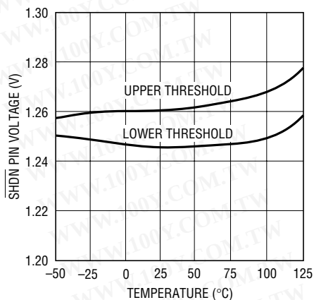
SHDN Pin Lockout Thresholds vs Temperature
