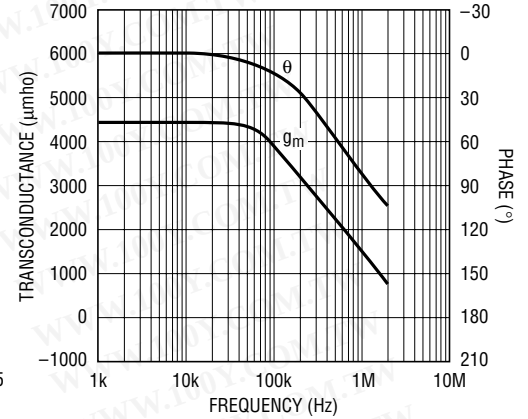
Transconductance of Error Amplifier
