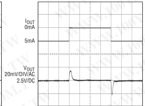
2.5V Load Transient Response (Sourcing)
