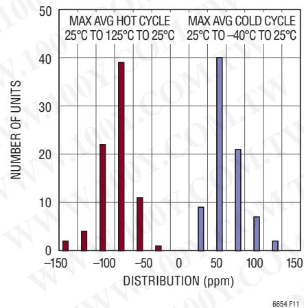
Figure 11. Thermal Hysteresis -40°C to 125°C
