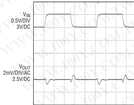
2.5V Line Transient Response
