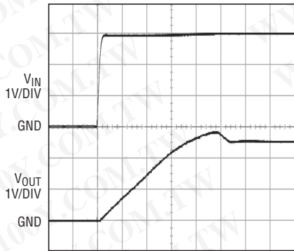
2.5V Turn-On Characteristics
