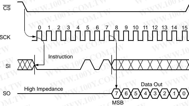
FIGURE 6. READ STATUS REGISTER SEQUENCE
