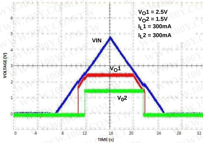
FIGURE 10. POWER-UP/POWER-DOWN
