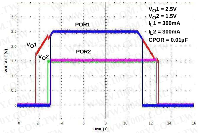
FIGURE 11. POWER-UP/POWER-DOWN WITH POR SIGNALS
