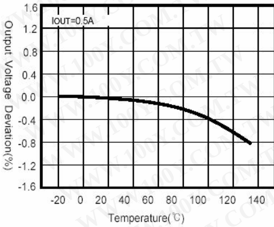
Temperature Stability
