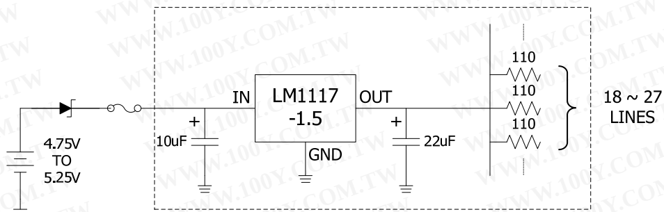
Fig.4 Active Terminator for SCSI-2BUS
