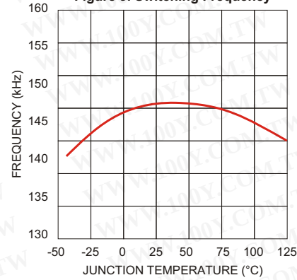
Figure 9. Switching Frequency
