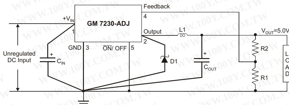
Figure 1(b). Adjustable Output Voltage Versions
