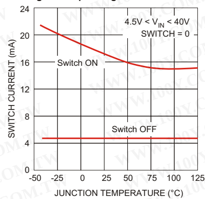
Figure 5. Operating Quiescent Current
