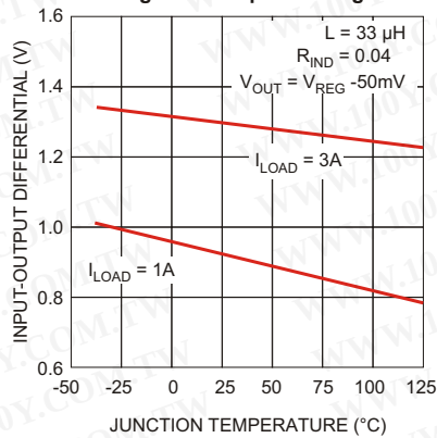
Figure 4. Dropout Voltage
