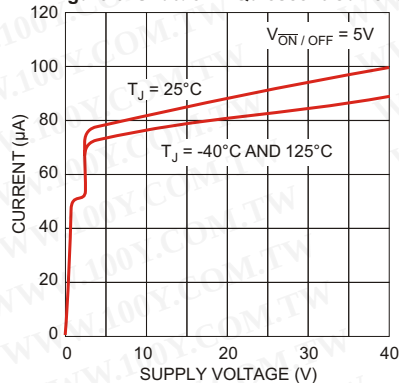
Figure 6. Shutdown Quiescent Current
