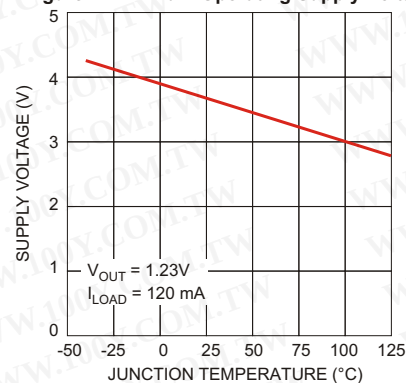
Figure 7. Minimum Operating Supply Voltage
