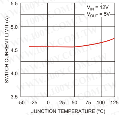
Figure 3. Switch Current Limit
