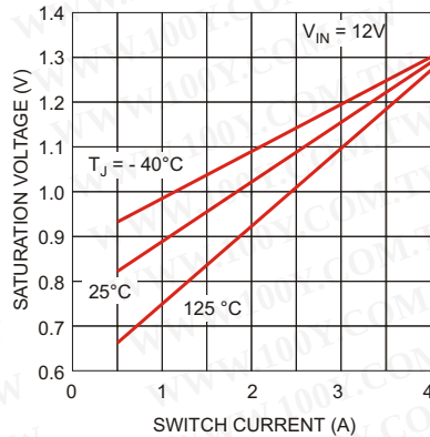
Figure 2. Switch Saturation Voltage
