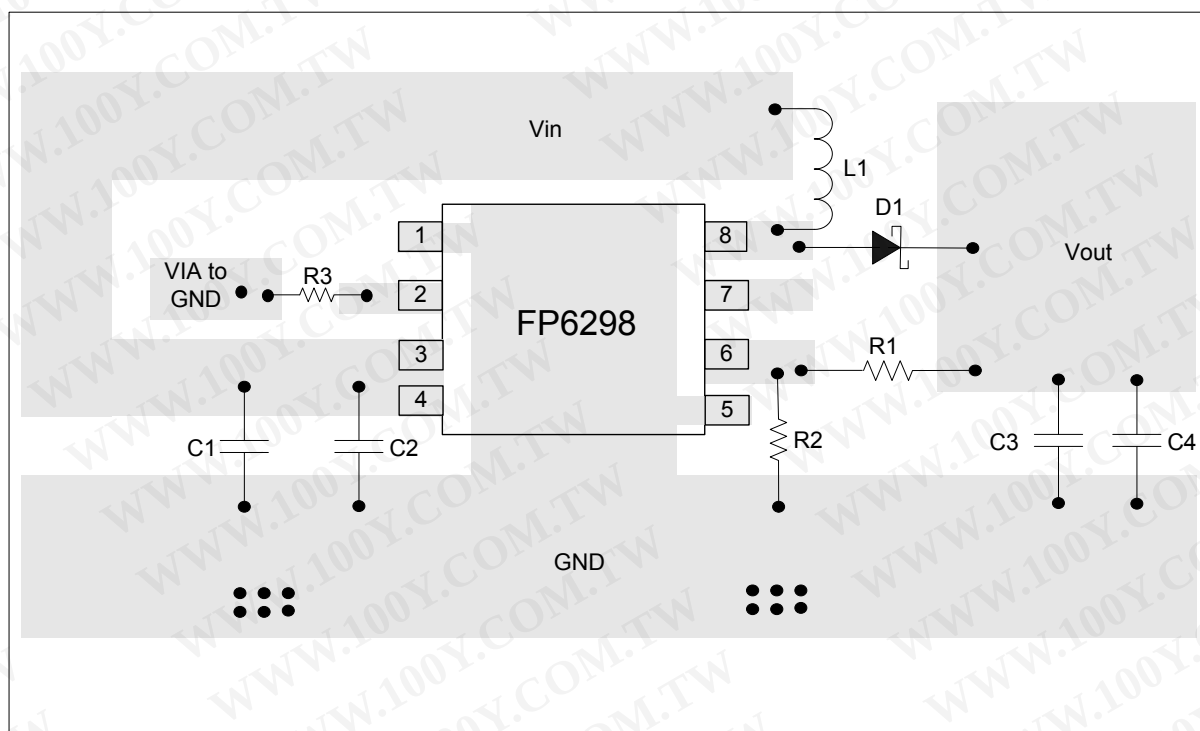
Suggested Layout
