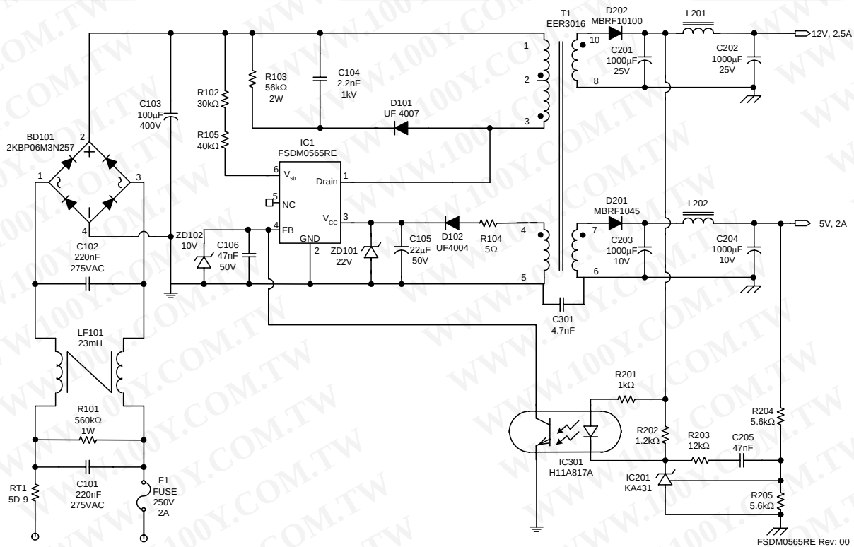
Figure 22. Demo Circuit
