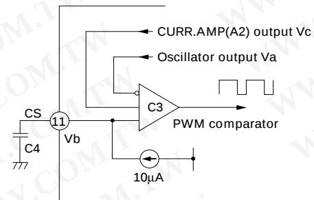
Fig. 5 PWM comparator
