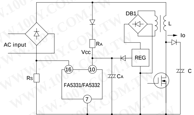
Fig. 9 Start circuit
