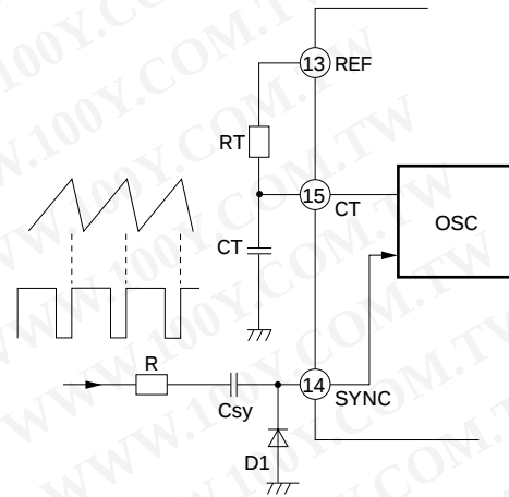
Fig. 1 Oscillator
