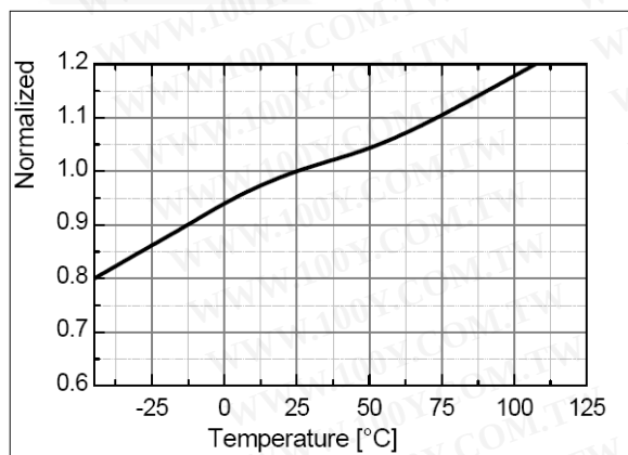
Figure 23. Output Saturation Voltage ( V_{RDY, SAT} ) vs. T_A
