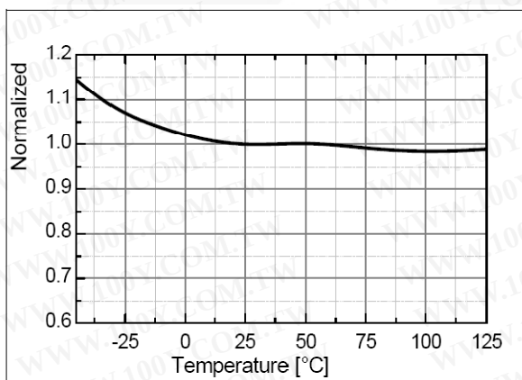
Figure 21. Restart Timer Delay ( t_{RST} ) vs. T_A
