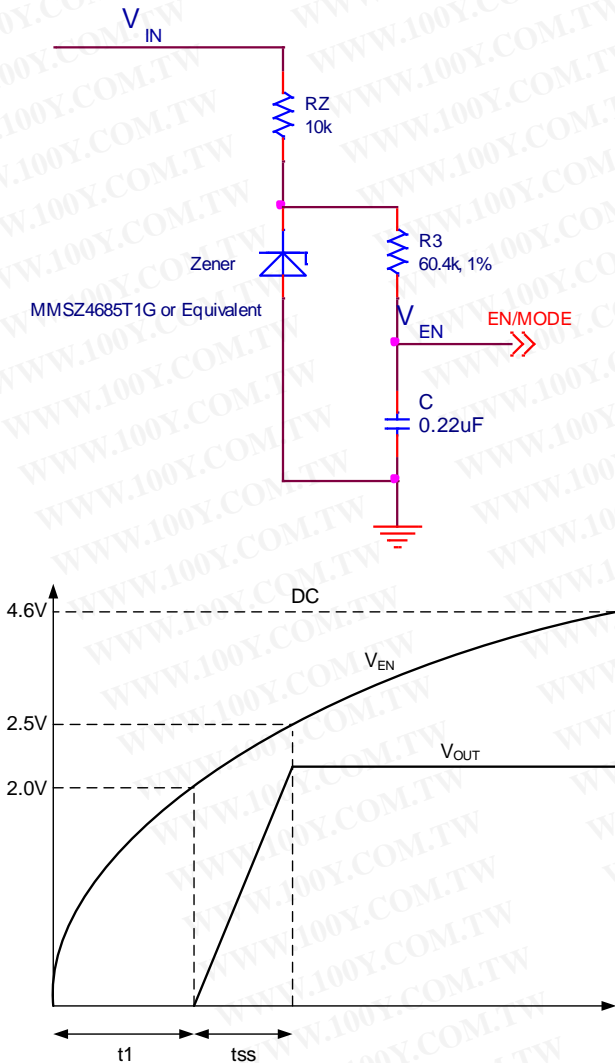
Figure 35: Timing circuit and diagram for selecting DCM/CCM by deriving EN/MODE from V_{IN}
