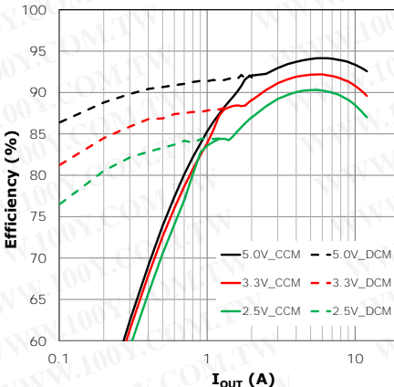
Figure 28: XR76112, 22V IN , 400kHz, 2.2uH
