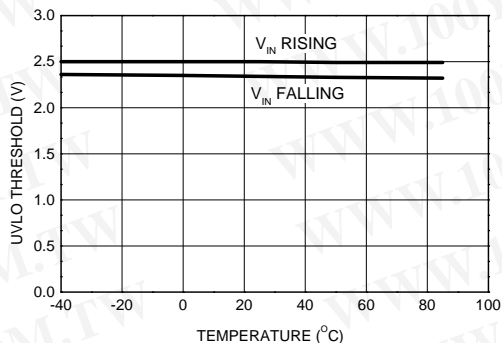
UVLO Threshold vs. Temperature
