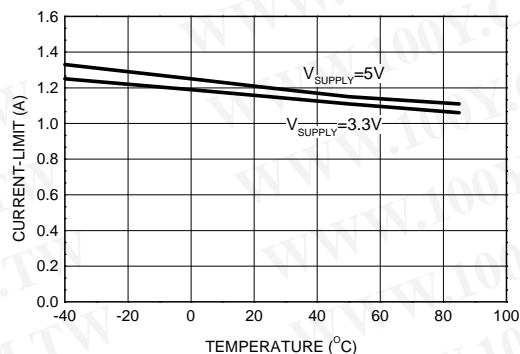
Current-Limit Threshold vs. Temperature
