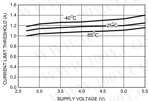
Current-Limit Threshold vs. Supply Voltage
