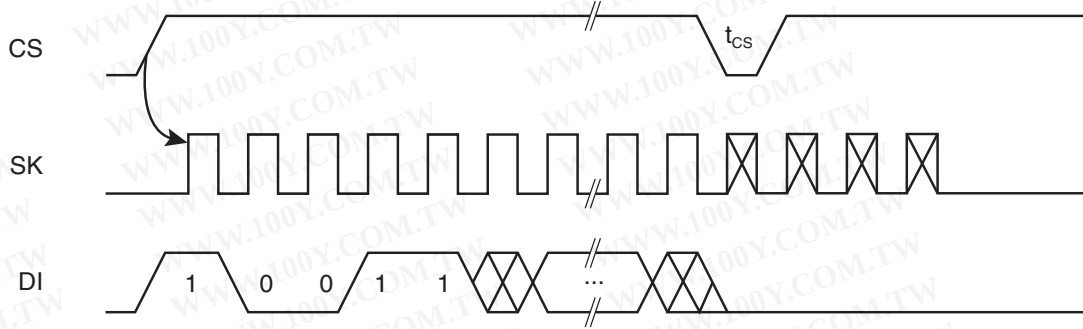
Figure 3-3. EWEN Timing
