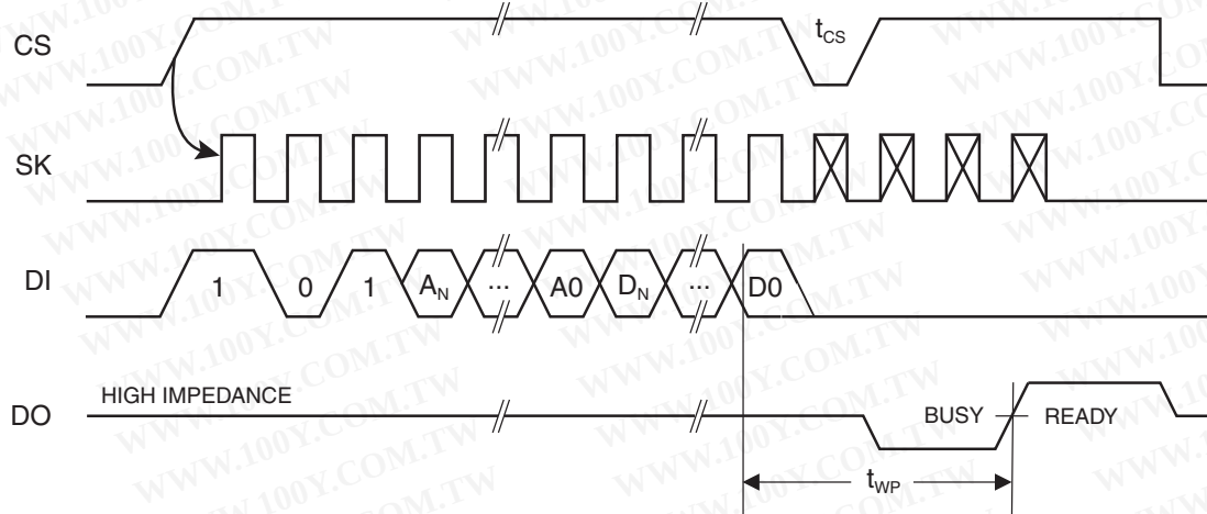
Figure 3-5. WRITE Timing
