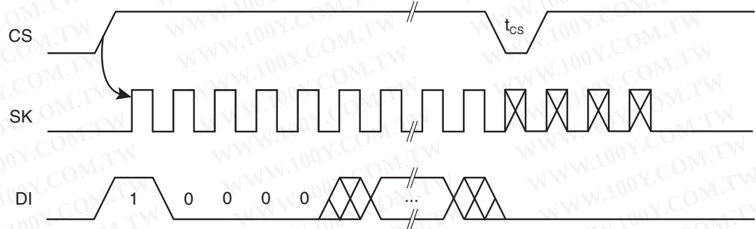
Figure 3-4. EWDS Timing
