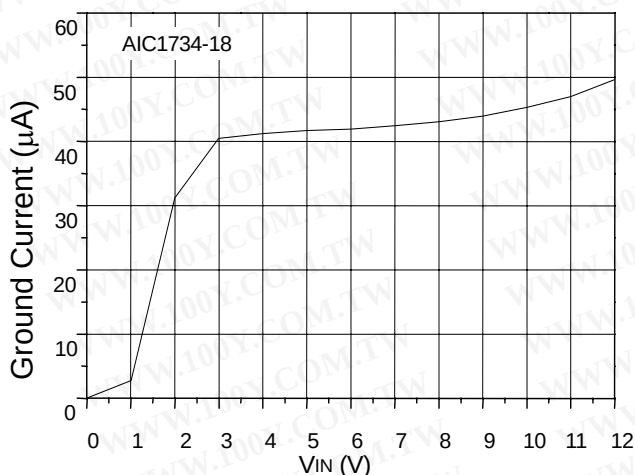
Fig. 9 Ground Current vs. V_{\text{IN}}
