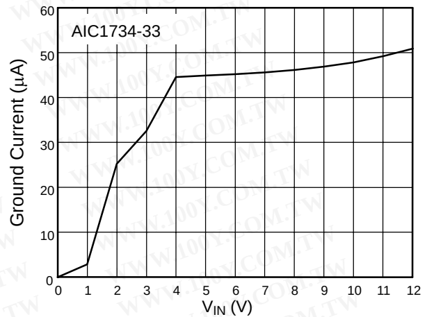
Fig. 8 Ground Current vs. V_{\text{IN}}
