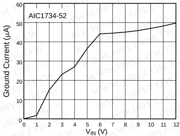
Fig. 7 Ground Current vs. V_{\text{IN}}
