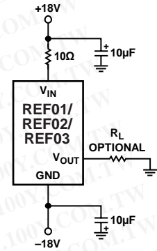
Figure 37. Burn-In Circuit
