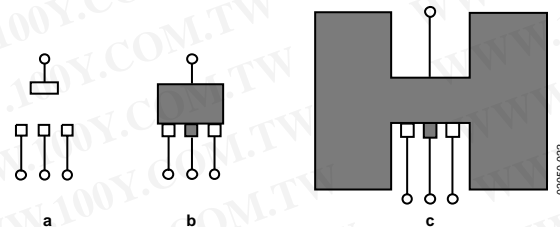
Figure 22. PCB Layouts
