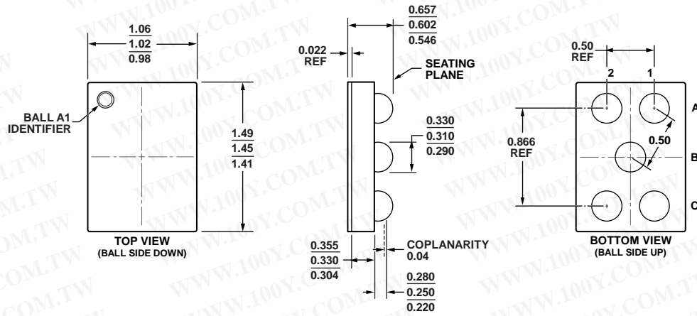
Figure 36. 5-Ball Wafer Level Chip Scale Package [WLCSP] (CB-5-3)
