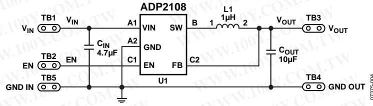
Figure 31. Evaluation Board Schematic
