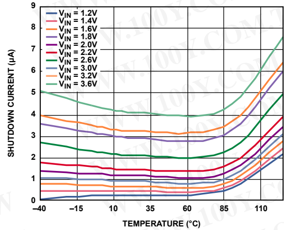
Figure 19. Reverse Output Shutdown Current vs. Temperature
