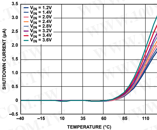
Figure 18. Reverse Input Shutdown Current vs. Temperature
