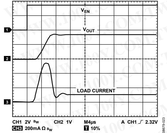
Figure 28. Typical Rise Time and Inrush Current, C_{LOAD} = 1\mu F, V_{IN} = 1.8V, \text{Load} = 200mA
