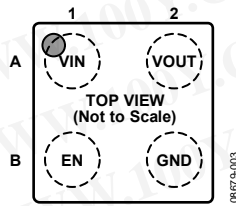
Figure 3. 4-Ball WLCSP Pin Configuration
