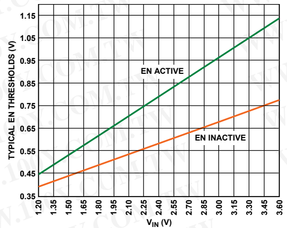
Figure 25. Typical EN Thresholds vs. Input Voltage ( V_{IN} )
