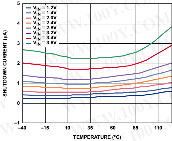
Figure 17. Shutdown Current vs. Temperature
