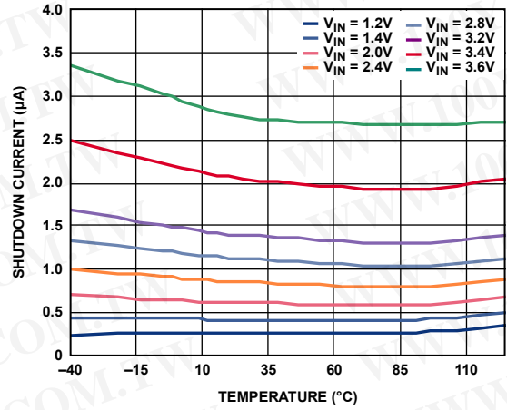
Figure 20. Reverse Shutdown Current vs. Temperature
