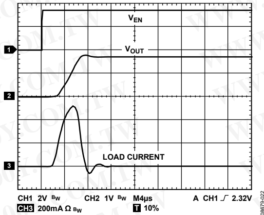
Figure 27. Typical Rise Time and Inrush Current, C_{LOAD} = 1\mu F, V_{IN} = 1.8V, \text{No Load}
