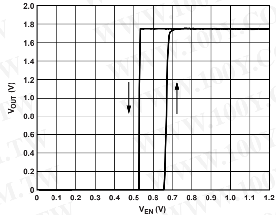
Figure 24. Typical EN Operation
