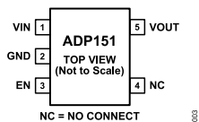
Figure 4. 5-Lead TSOT Pin Configuration
