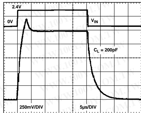
Figure 19. Turn-On Response Time
