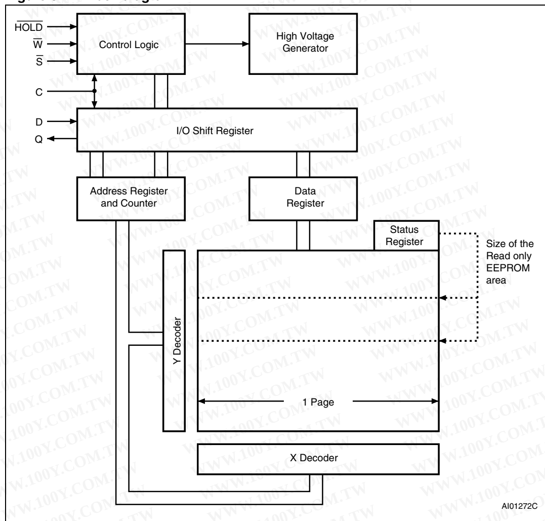
Figure 6. Block diagram
