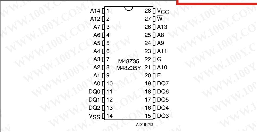
Figure 2. DIP connections
