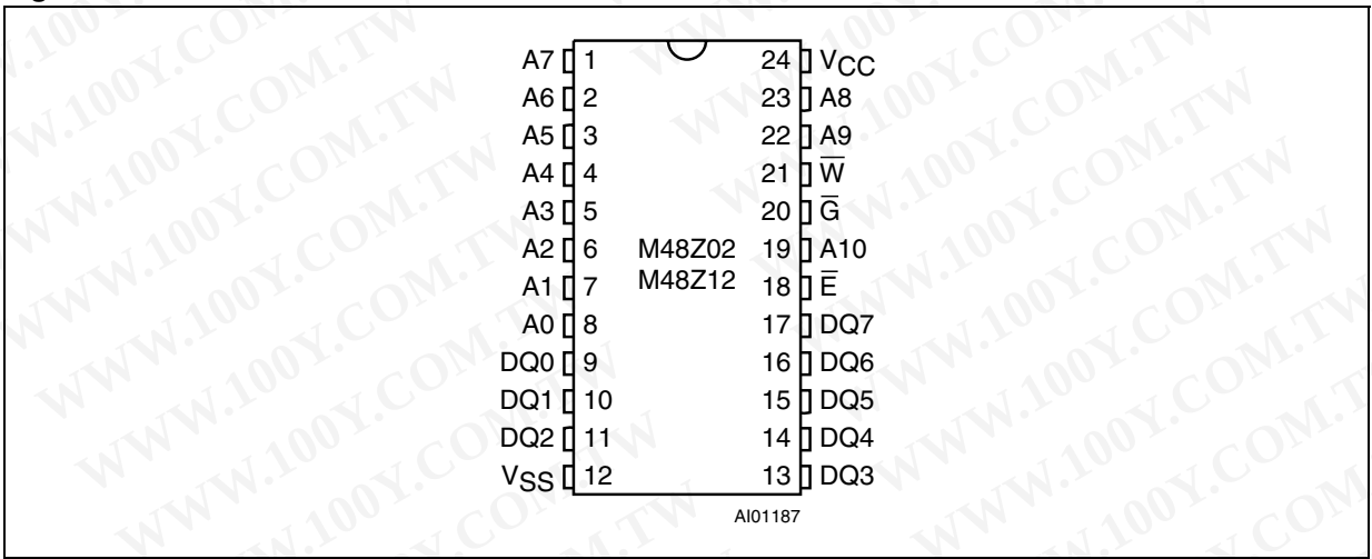
Figure 2. DIP connections
