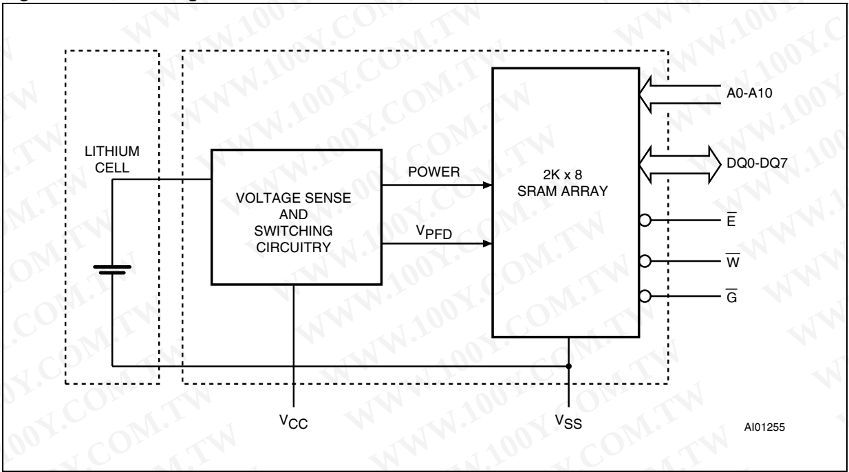
Figure 3. Block diagram
