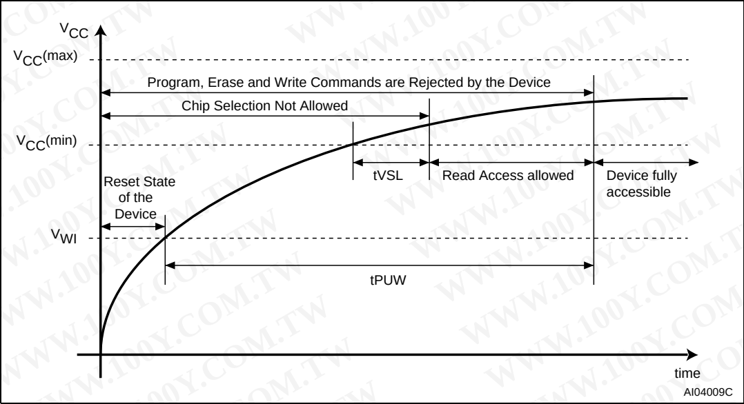
Figure 18. Power-up timing
