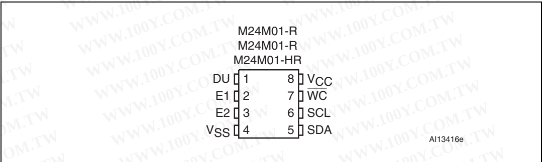
Figure 2. SO connections
