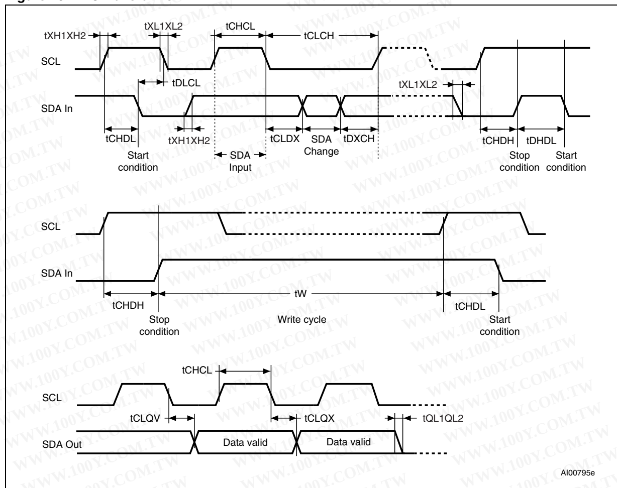
Figure 13. AC waveforms
