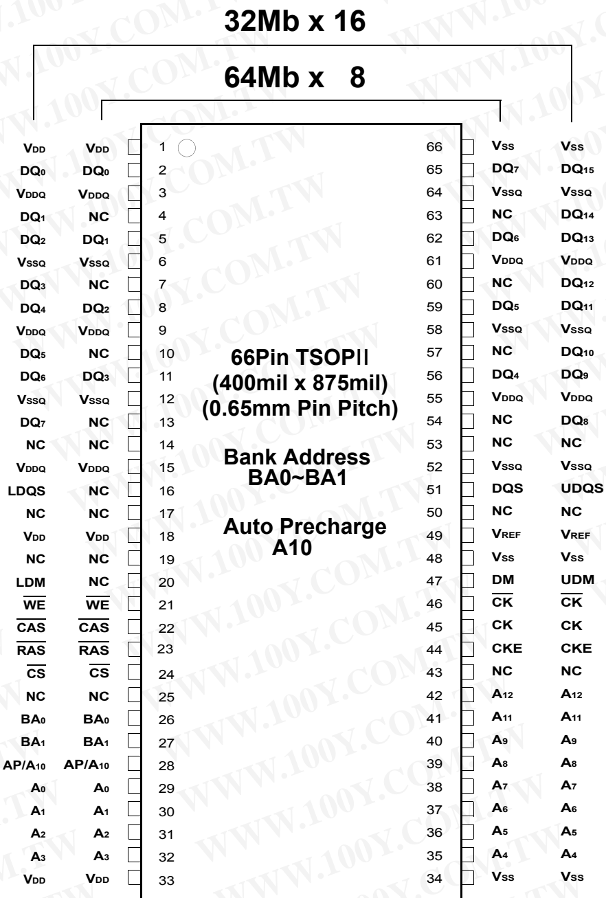
512Mb TSOP-II Package Pinout
