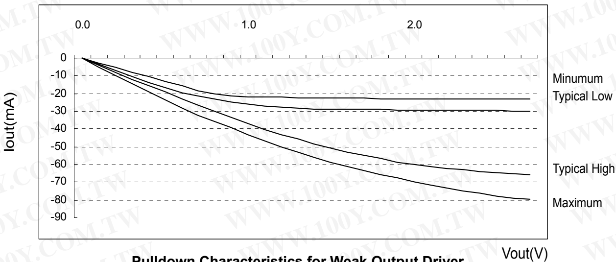
Pulldown Characteristics for Weak Output Driver
