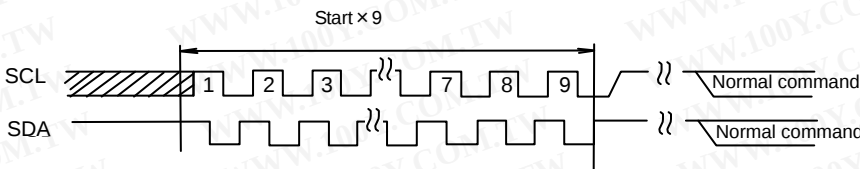
Fig.48-(c) START×9+ command input
