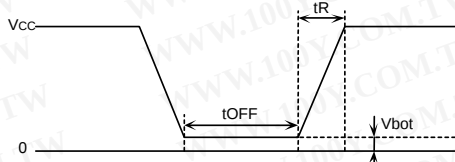
Fig.59 Rise waveform diagram
