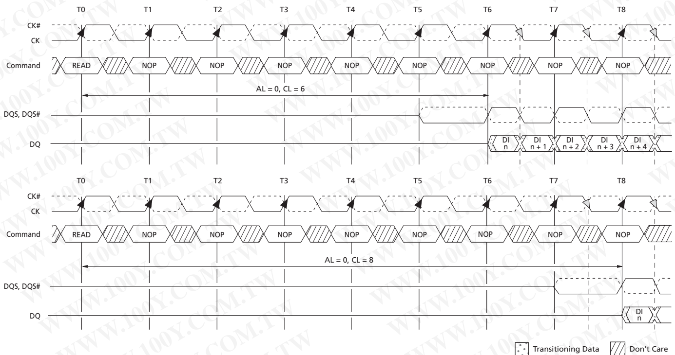
Figure 47: READ Latency
