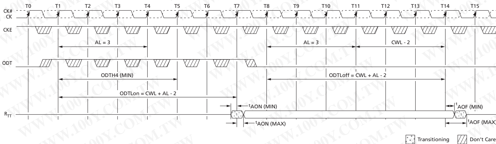
Figure 108: Synchronous ODT
