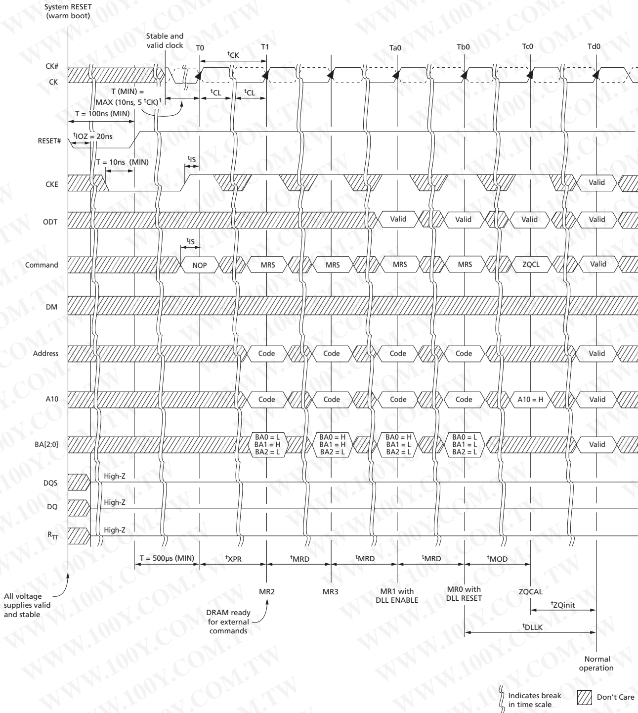
Figure 101: RESET Sequence
