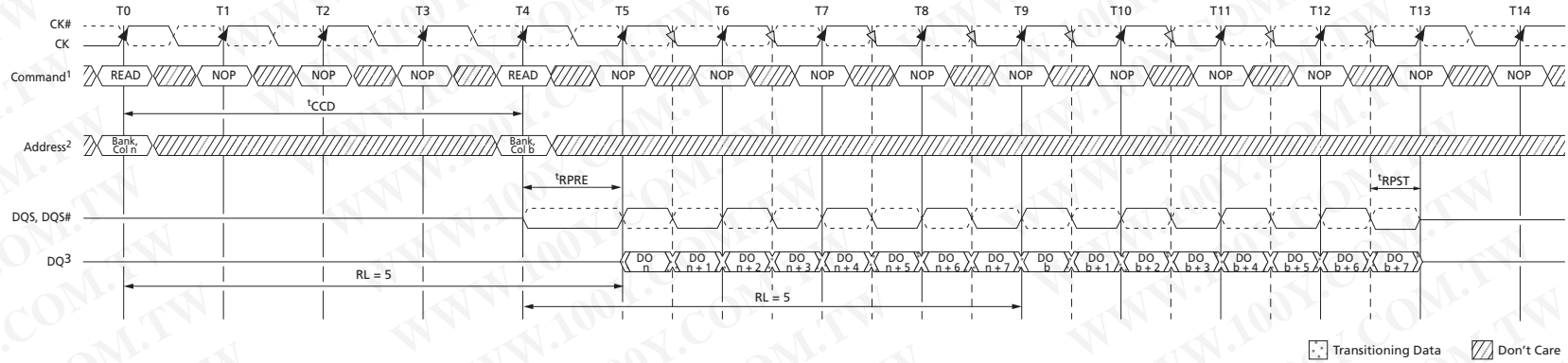
Figure 62: Consecutive READ Bursts (BL8)
