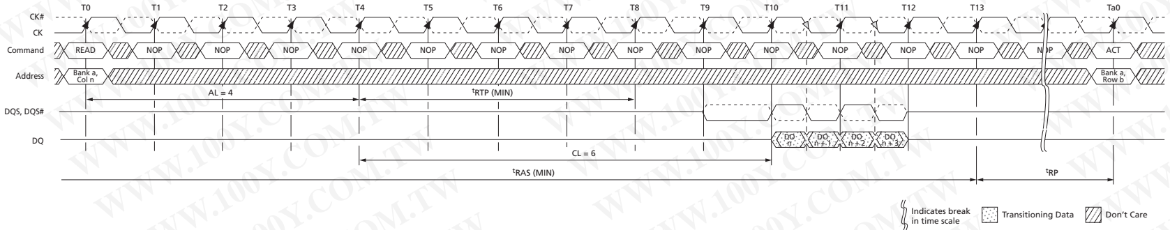
Figure 70: READ with Auto Precharge (AL = 4, CL = 6)
