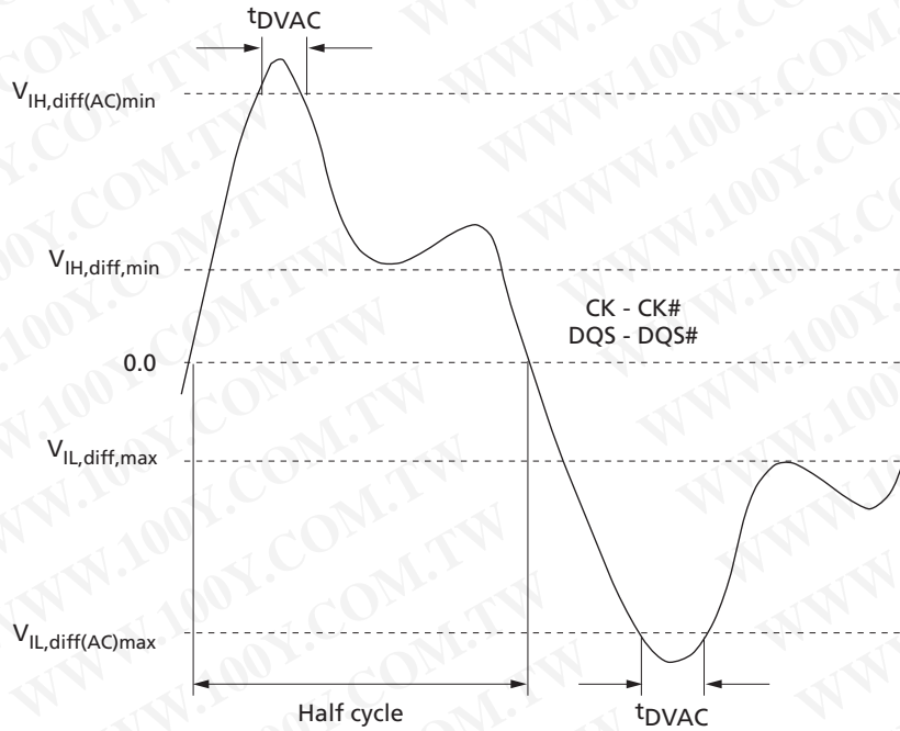
Figure 18: Definition of Differential AC-Swing and t_{DVAC}
