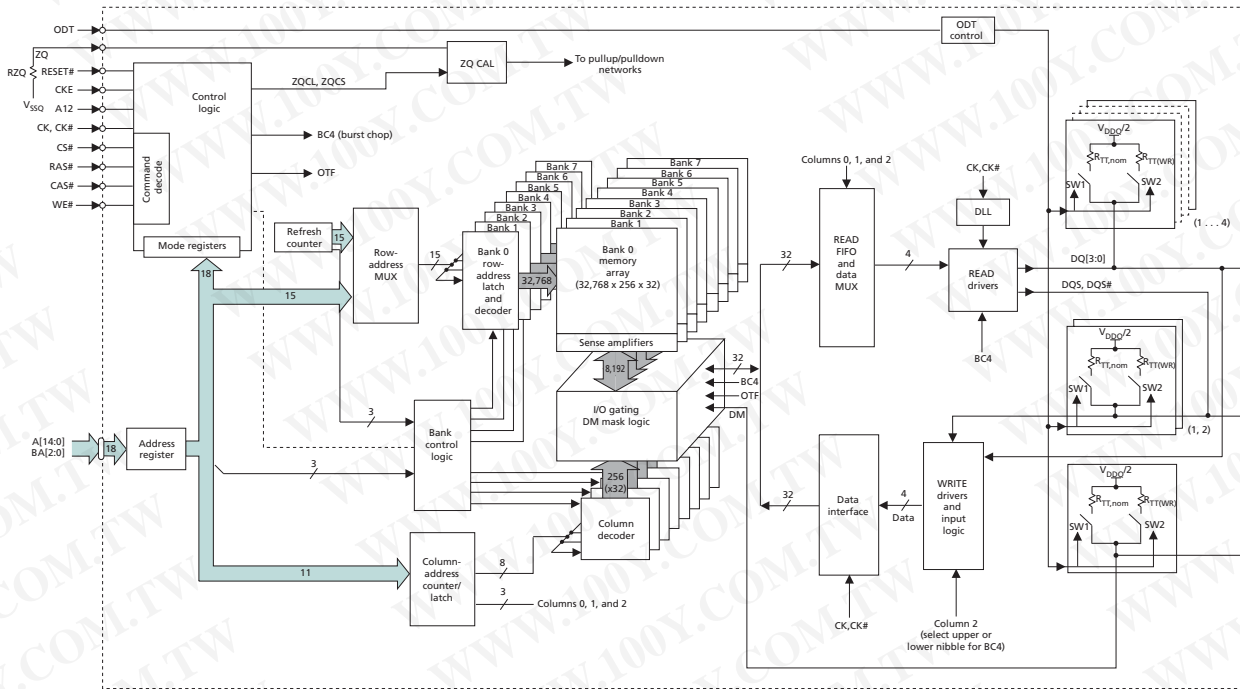
Figure 3: 512 Meg x 4 Functional Block Diagram
