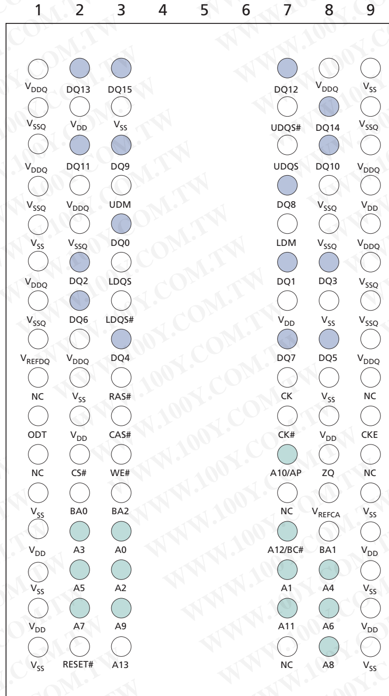
Figure 7: 96-Ball FBGA – x16 (Top View)
