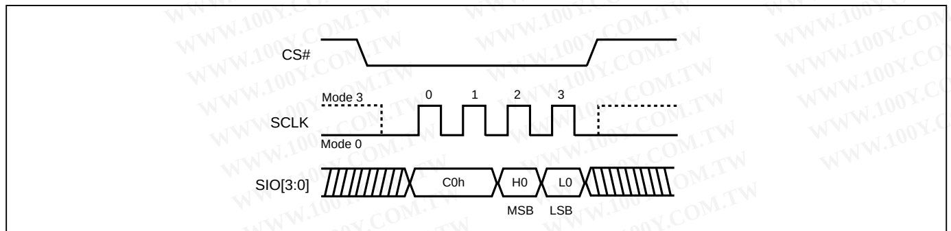
Figure 34. QPI Mode
