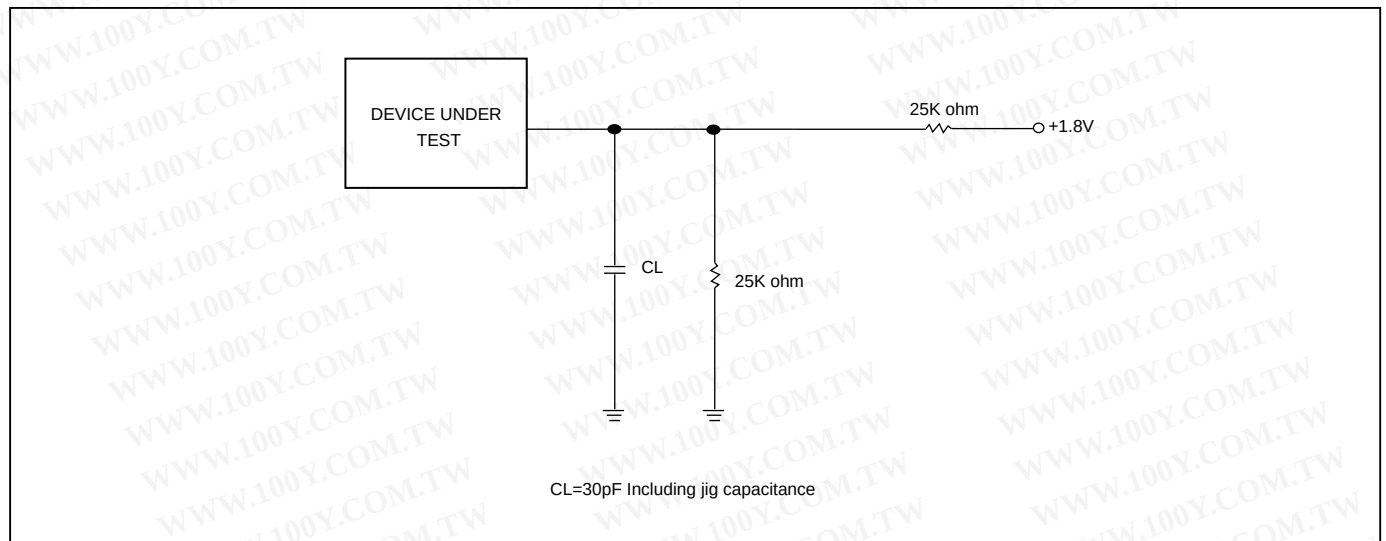
Figure 66. Output Loading
