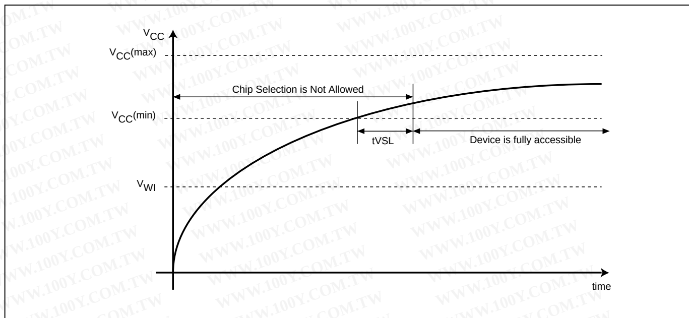
Figure 69. Power-up Timing
