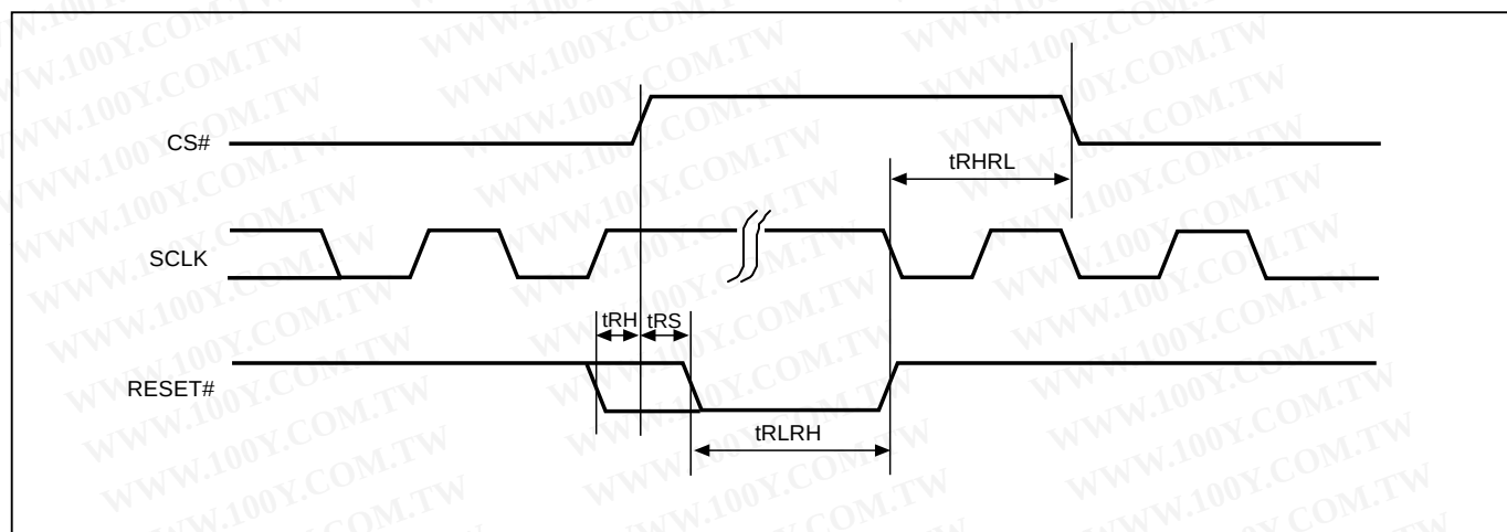
Figure 62. RESET Timing
