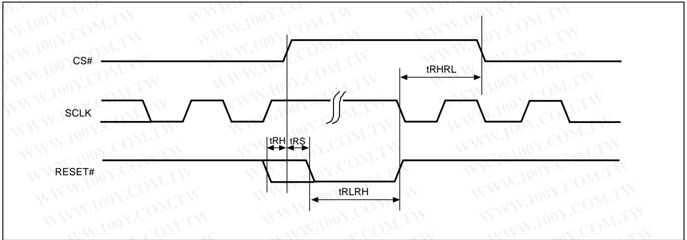
Figure 61. RESET Timing
