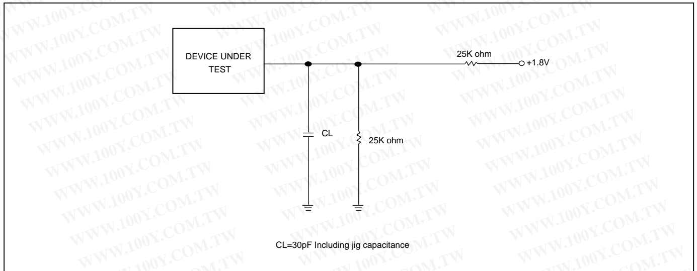
Figure 65. OUTPUT LOADING
