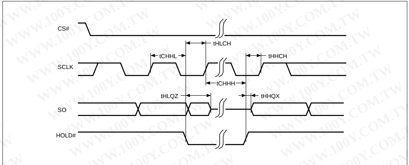
Figure 9. Hold Timing
