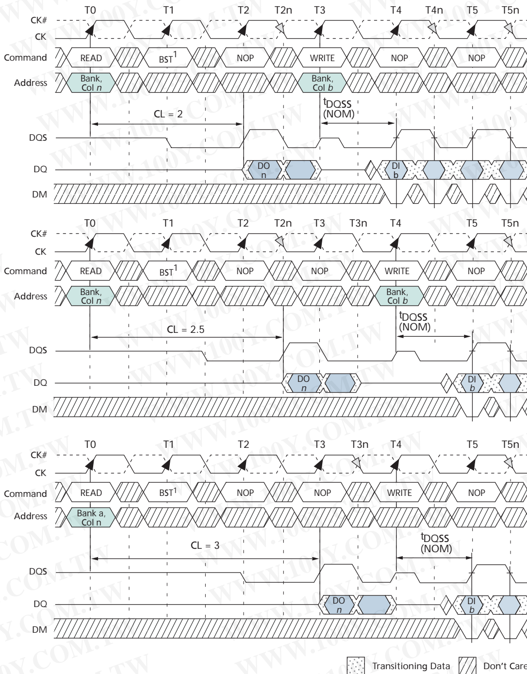
Figure 32: READ-to-WRITE
